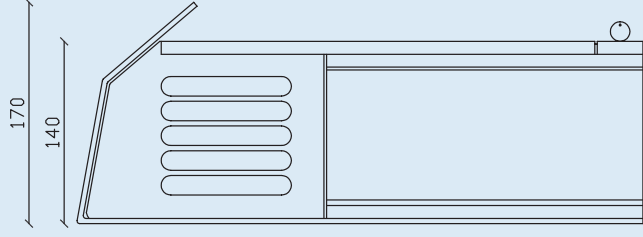
SIDE ELEVATION (ashtray slide in closed position )
