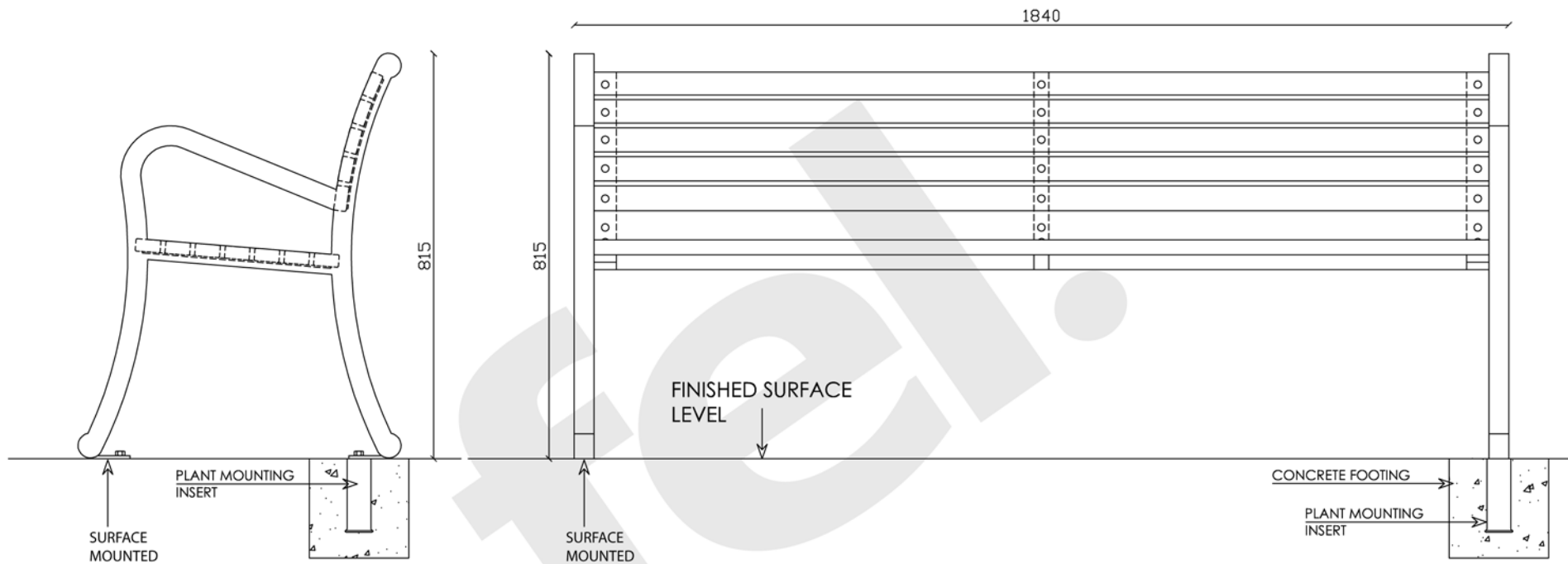
FRONT ELEVATION
